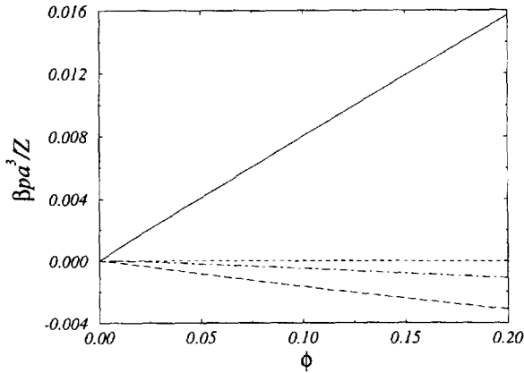
Fig. 3. Dependence of the various contributions to the dimensionless (total) pressure, \beta p a^3 / Z , on the volume fraction \phi = (4/3)\pi a^3 \rho_p , for Z = 1000 , and T^* = 100 . Solid line: mixing (ideal-gas) contribution; long-dashed line: polyion-counterion contribution; dot-dashed line: polyion-polyion contribution; dashed line: counterion-counterion contribution.
