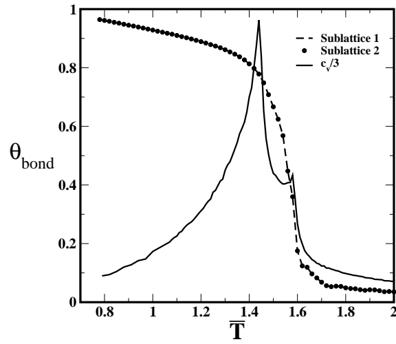
FIG. 8: Order parameter and specific heat vs. temperature for chemical potential \bar{\mu} = 1 and lattice size L = 30 . As can be seen, both sublattices orders itself in one arm configuration when cross the \tau -line.
