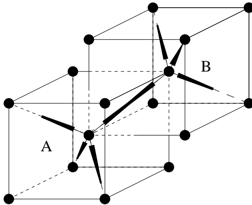
FIG. 1: Particles in the BCC lattice can assume arms configuration A or B.
