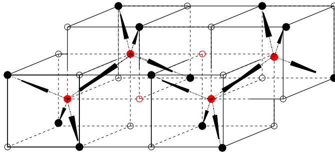
FIG. 2: In the ordered low density liquid phase half of the lattice is occupied by particles.
