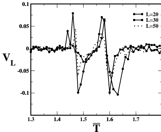
FIG. 6: Cumulant of energy vs. reduced temperature for reduced chemical potential \bar{\mu} = 1 and lattice sizes L = 20, 30 and 50 .
