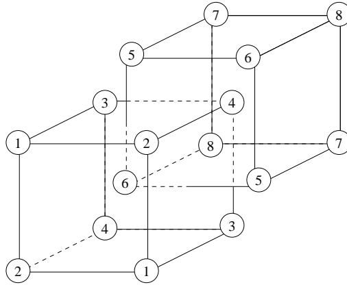
FIG. 9: The 8 sublattices division. Sublattices 1,4,6,7 become occupied, while the other sublattices become empty. Particles on sublattice 1 and 4 orient mostly in the A state, while particles on sublattice 6 and 7 orient into the B state.
