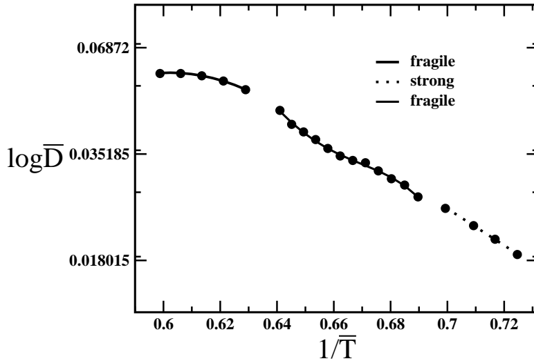
FIG. 12: Diffusion coefficient as a function of temperature in an Arrhenius plot for \bar{\mu} = 1.0 . For temperatures T > T_\tau diffusivity follows a non-Arrhenius law, characterizing the liquid as fragile. At temperatures T_\lambda < T < T_\tau , the liquid is also characterized as fragile since diffusivity follows a non-Arrhenius law. For temperatures T < T_\lambda diffusivity follows an Arrhenius law, and the liquid is characterized as strong.
