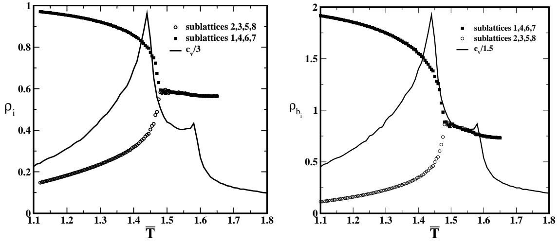
(a) Density of particles for the eight sublattices and specific heat vs. reduced temperature for \bar{\mu} = 1 . At the \lambda -line four sublattices become empty while the other four become full. The specific heat is also shown for illustrating the location of the \lambda -line. (b) Density of bonds versus reduced temperature for eight sublattices \bar{\mu} = 1 . Four sublattices have all the empty sites with bonds while the other four have no bonds. The specific heat is also shown for illustrating the location of the \lambda -line.
