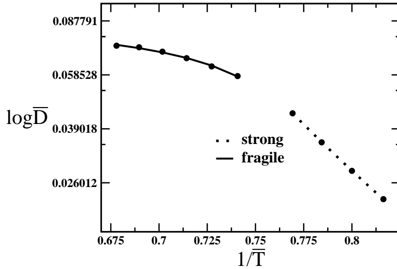
FIG. 11: Diffusion coefficient in an Arrhenius plot for \bar{\mu} = 0 . At high temperatures, diffusivity follows a non-Arrhenius law, while at low temperatures diffusivity follows an Arrhenius law. The dynamic crossover takes place when the system crosses the coexistence line between the Gas-LDL phases.
