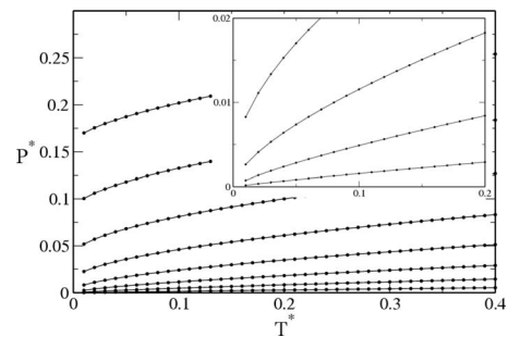
FIG. 3. Phase diagram in Rogers-Young integral equations. The low isochores \rho = 0.01, 0.02, 0.03, 0.04, 0.05, 0.06, 0.07 , and 0.08 , from bottom to top, are shown. The inset shows the isochores for \rho^* = 0.01, 0.02, 0.03 , and 0.04 . For \rho^* \leq 0.03 , the isochores are converging to a point at the supercooled region—the liquid-gas phase transition.
