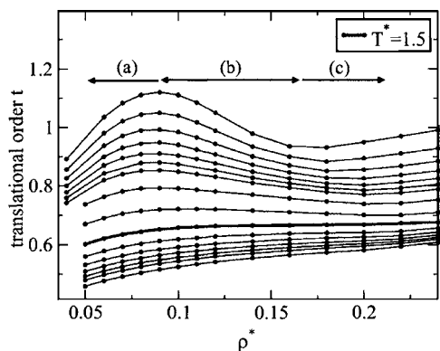
FIG. 4. The translational order parameter t as a function of the density \rho^* . From top to bottom, the 16 isotherms are T^* = 0.25, 0.30, 0.35, 0.40, 0.45, 0.50, 0.55, 0.70, 1.0, 1.5, 2.0, 2.5, 3.0, 3.5, 4.0, and 5.0 . The arrows (a), (b), and (c) correspond to the density range spanned by Figs. 5(a)–5(c), respectively. The bold line indicates the isotherm T^* = 1.5 . For T^* > 1.5 no anomalous behavior is observed for t . The line connecting the points is just a guide for the eyes.
