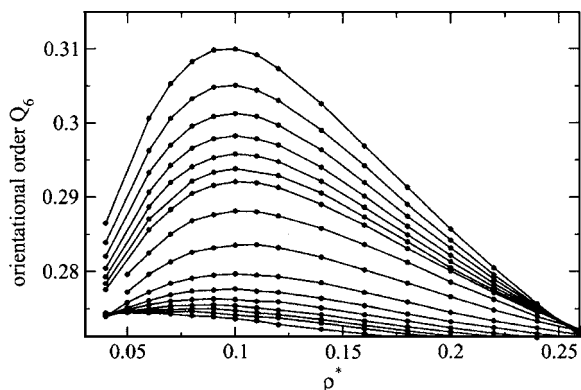
FIG. 6. The orientational order parameter Q_6 as a function of the density \rho^* . From top to bottom, the 16 isotherms are T^*=0.25, 0.30, 0.35, 0.40, 0.45, 0.50, 0.55, 1.0, 1.5, 2.0, 2.5, 3.0, 3.5, 4.0, and 5.0 . For 5.0 < T^* < 8.0 (not shown) the Q_6 local maximum points occur at \rho^*=0 with a global minimum at \rho^*\approx 0.3 . We do not study the cases where T^* > 8.0 (see the text for more details). The line connecting the points is just a guide for the eyes.
