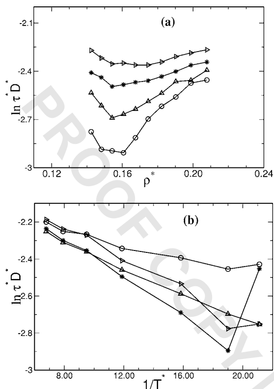
FIG. 6. (a) Product \tau_r D_r^* as a function of density for four isotherms (from top to bottom T^*=0.105, 0.084, 0.063, and 0.052 ) for n=144 steps (b) Product \tau_r D_r^* as a function of the inverse of temperature along isochores for n=144 steps (circles: \rho=0.208 , up triangles: \rho=0.175 , stars: \rho=0.154 , right triangles: \rho=0.142 ).
