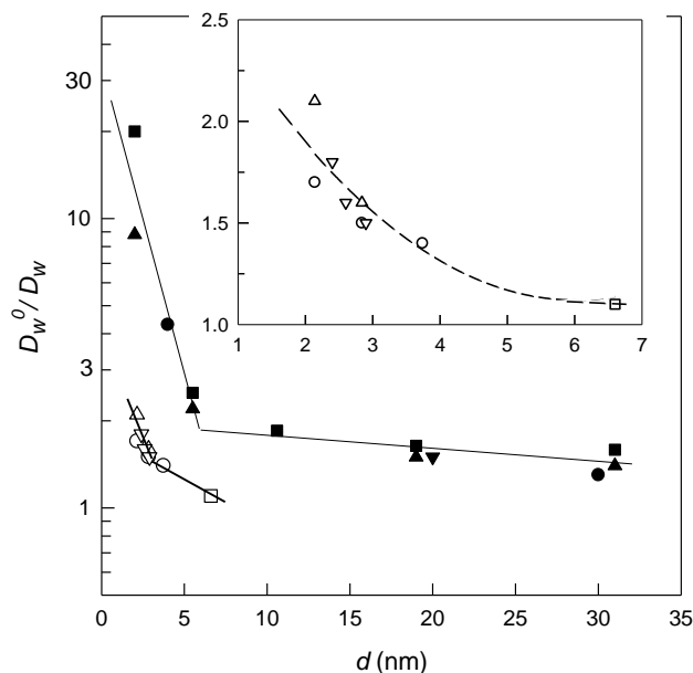
Figure 14. Tortuosity factor for the diffusion of water in ordered (empty symbols) and disordered (full symbols) silica as a function of the pore size: (●) Vycor/Bioran glass [292]; (▲) CARIAC [293]; (■) CARIAC [296]; (▼) GelSil [297]; (○) MCM-41 [298], (Δ) MCM-41 [299]; (▽) MCM-41 [304]; (□) SBA-15 [303]. The inset shows a zoom of the small pore ordered silica, and the lines are a guide for the eye.
