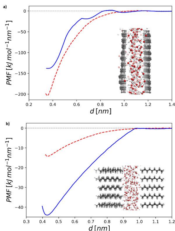
Figure 19. Potential of mean force (PMF) as a function of the separation between (a) two graphene sheets and (b) two self-assembled monolayers. In both figures, full lines correspond to the PMF calculated in TIP3P water while dashed lines correspond to the PMF obtained in vacuum.
