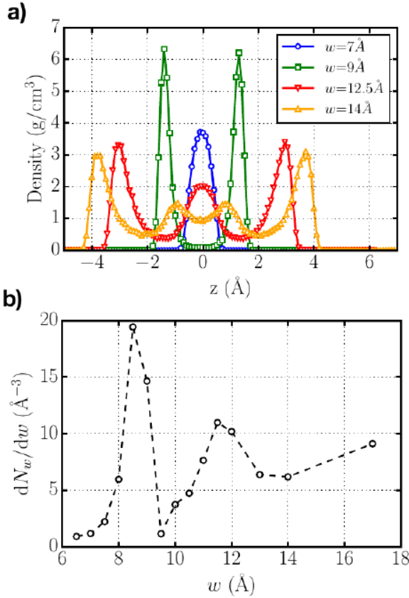
Figure 10. (a) Water density profile as a function of the distance, z , from the center of the nanoconfined region between the plates, for different slit-pore widths, w/\text{\AA} = 7, 9, 12.5 and 14 . (b) Variation of the internal slit-pore hygroscopicity, i.e., the derivative of the number of water molecules, N_w , in the analyzed central region (see text), as a function of w . Adapted from Ref. 196 with permission from Elsevier.
