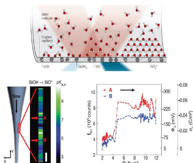
Figure 5. The H_2O layers and surface charge at a confined water-silica interface of a glass capillary can be mapped with micrometer resolution using x-ray spectroscopies. The top panel displays a cartoon of the aqueous phase for different surface states of charge. The lower panel presents the pK_a values obtained along the longitudinal axis of the capillary, together with curves of the surface potential and charge versus bulk pH at the two spots marked A and B on the left bottom image. Reproduced from Refs. 114 and 115 with permission of the American Association for the Advancement of Science.
