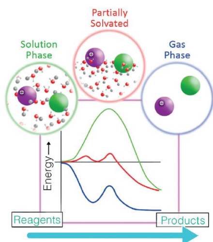
Figure 2. Schematics of the free-energy profiles for a reaction involving an ionic species in the bulk and gas phases, and under confinement in a small droplet. The large surface/volume ratio favors desolvation thus lowering the activation barrier. Reproduced from Ref. 81 with permission of John Wiley & Sons.
