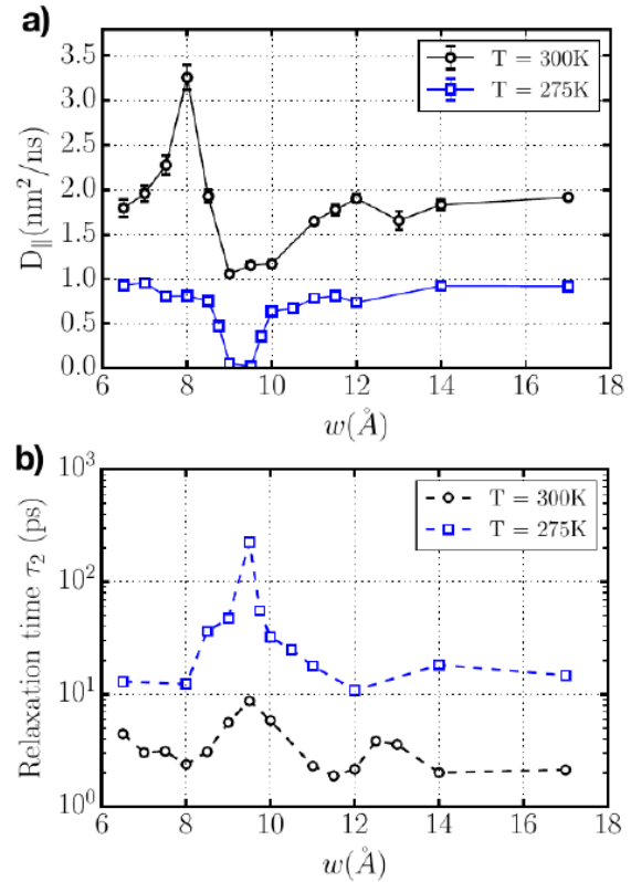
Figure 11. Dynamics of confined water molecules as a function of graphene-plate distance w at T = 300 \text{ K} and T = 275 \text{ K} . (a) Diffusion coefficient parallel to the plates D_{||} . (b) Reorientation relaxation time \tau_2 . Adapted from Ref. 196 with permission from Elsevier.
