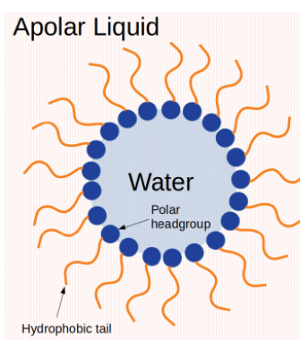
Figure 3. Representation of a reverse micelle consisting of a core of water stabilized in a non polar solvent by amphiphile molecules. These kinds of structures can be found in microemulsions, with sizes typically ranging from 1 to 100 nm depending on the water/organic ratio and surfactant concentration.
