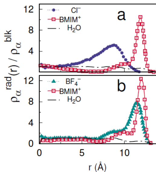
Figure 17. Normalized radial density fields for different species of confined RTILs within hydrophobic pores of radius R = 12.5 Å. Adapted with permission from Ref. 368. Copyright 2018 American Chemical Society.
