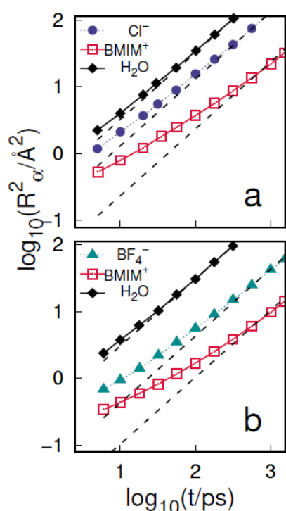
Figure 18. Mean square displacements, R^2 , for different species of confined RTILs solutions within pores of radius R = 12.5 \text{ \AA} . Individual diffusion coefficients were computed from the limiting slopes of the mean square displacement (MSD), i.e., D = \lim_{t \rightarrow \infty} (R^2(t)/2t) . The dashed lines correspond to asymptotic linear plots, with slope one. The MSDs of the confined ions remain in the sublinear temporal regime over time spans unusually long for standard liquid phases. Given the characteristics of the wall-solvation states already described, the sublinear temporal regime might reflect the presence of mechanisms akin to highly correlated “single-file-diffusion” motions, in which surpassing episodes between different particles are severely hindered. Adapted with permission from Ref. 368. Copyright 2018 American Chemical Society.
