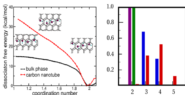
Figure 6. Left panel: free-energy profiles for the dissociation of water in bulk (black) and confined in a (6,6) carbon nanotube (red), computed from first-principles Car-Parrinello molecular dynamics using the coordination number as the reaction coordinate: 2 and 1 correspond to initial state and final dissociated state, respectively (see text). Configurations sampled along the reaction coordinate are depicted in the insets. Right panel: Histogram of the number of hydrogen bonds formed by the hydronium and the hydroxide ions. Blue: hydronium in the bulk phase. Red: Hydroxide in the bulk phase. Green: hydronium in the nanotube. Indigo: hydroxide in the nanotube. Reproduced with permission from Ref. 148. Copyright 2018 American Chemical Society.
