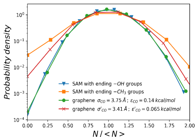
Figure 20. Probability distributions for observing N water molecules within a small spherical observation volume of radius 3.3 Å (similar to a methane molecule) tangent to the different surfaces studied.
