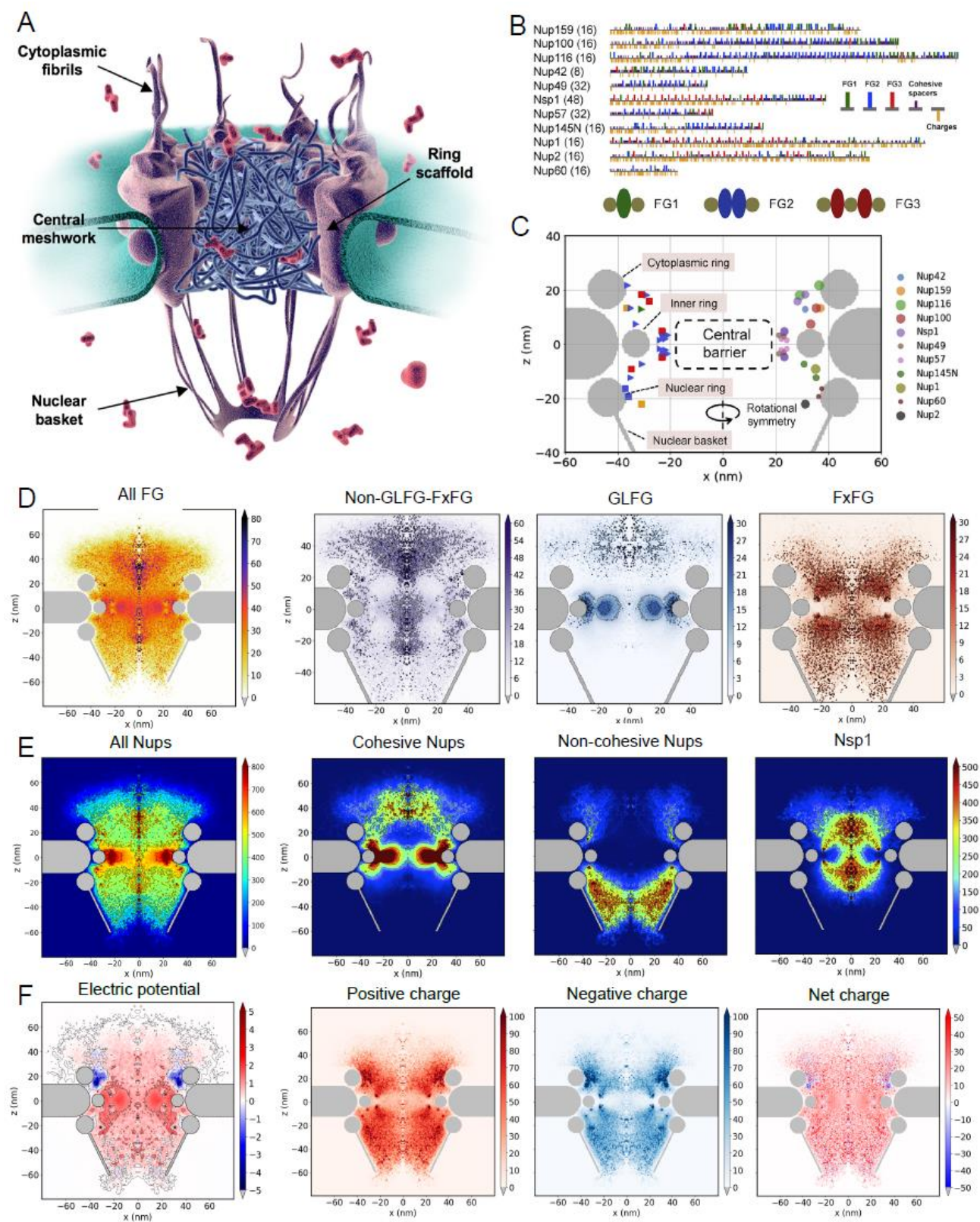
Figure 25. Molecular theory of the yeast NPC. (A) Schematic representation of the NPC. Reprinted with permission from Ref. 523. (B) Stoichiometry and Amino-acid sequences of the FG-Nups. (C) Coarse-grained scaffold structure and anchor positions of the FG-Nups. (D) Spatial distributions of FG groups. (E) Spatial distribution of FG-Nups. (F) Electric potential and charge distribution throughout the NPC. All the color maps for amino acid concentrations are in the units of mM. The color map for electric potential is in the units of mV. Reprinted with permission from Ref. 509, Copyright 2020 American Chemical Society.
