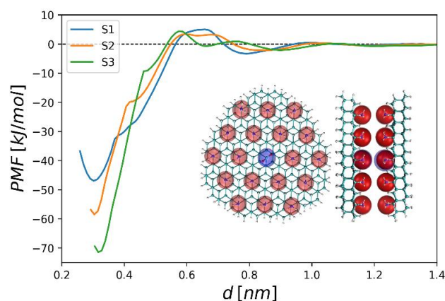
Figure 21. Potential of mean force in water (TIP3P) for the different simulated systems with charged group in the center of each surface ( \text{NH}_3^+ in one of them and \text{CO}_2^- in the other), as a function of the plate distance (the distances are measured between the positions of the charged groups of both plates): S1 for parallel surfaces with polar groups ( -\text{NH}_2 ) environment; S2 for parallel surfaces, one with apolar groups ( -\text{CH}_3 ) environment and the other with polar groups ( -\text{NH}_2 ) environment and S3 for parallel surfaces with apolar groups ( -\text{CH}_3 ) environment.
