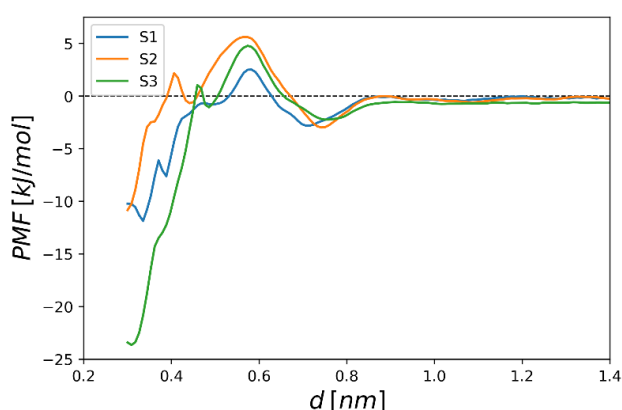
Figure 22. Arithmetic difference between the PMFs obtained for the charged and neutral systems in TIP3P water: S1 for parallel surfaces with polar groups ( -\text{NH}_2 ) environment; S2 for parallel surfaces, one with apolar groups ( -\text{CH}_3 ) environment and the other one with polar groups ( -\text{NH}_2 ) environment and S3 for parallel surfaces with apolar groups ( -\text{CH}_3 ) environment.
