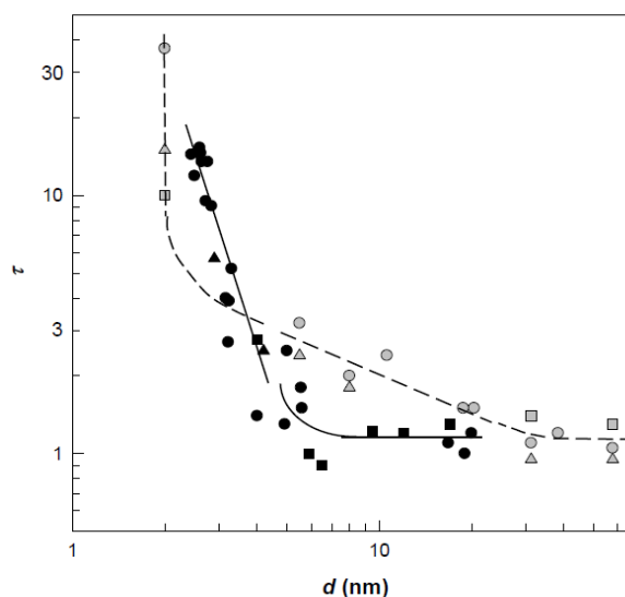
Figure 15. Tortuosity factor for the diffusion of aqueous ions confined in mesoporous silica. Symbols: \text{Li}^+ ( \bullet ), \text{K}^+ ( \blacktriangle ), and \text{Cs}^+ ( \blacksquare ) in CARIACT [296]; \text{Er}(\text{NO}_3)_3 and \text{Nd}(\text{NO}_3)_3 ( \blacktriangle ) [306] \text{Cr}(\text{NO}_3)_3 ( \bullet ) [312], and \text{Ni}(\text{NO}_3)_2 ( \blacksquare ) [308] in sol–gel glasses. The lines are a guide for the eye.
