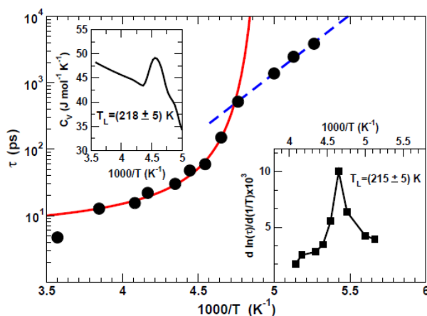
Figure 8. Main frame: \alpha -relaxation time \tau of the free water confined in MCM-41 silica as function of 1000/T . The continuous red line is the VFT fit via Eqn. 8. The dashed blue line is the Arrhenius fit via Eq. 3. The FSC takes place at T_L \sim 215 K. Upper Inset: specific heat of the system as function of 1000/T showing a peak at the FSC. Bottom Inset: inverse temperature derivative of \ln(\tau) , used to precisely locate the temperature of the FSC. Adapted with permission from Ref. 174. Copyright 2010 American Chemical Society.
