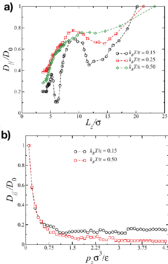
Figure 13. (a) Lateral diffusion constant normalized by the bulk diffusion as function of the walls separation for the CS fluid confined between fixed walls at distinct temperatures. (b) Lateral diffusion constant normalized by the bulk diffusion as function of the wall pressure for the CS fluid confined between oscillatory walls at distinct temperatures. Adapted from Ref. 197, with the permission of AIP Publishing.
