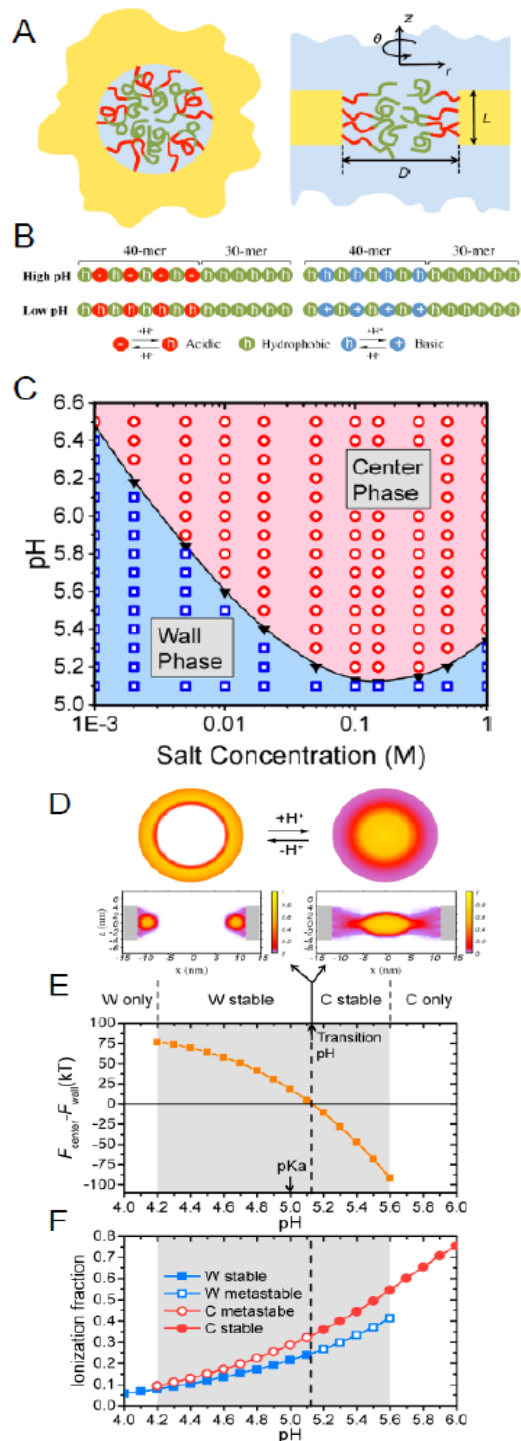
Figure 24. Design of copolymer for smart (stimuli-responsive) nanopore. (A) Schematic representation of the copolymer grafted short nanopore. (B) Sequence design of the copolymer. The copolymer contains in total 70 monomers, which can be classified into two groups according to their ionizability. The ionizable ones are hydrophilic as they get charged, and hydrophobic when they are neutral. (C) Phase diagram of the nanopore. (D) Switching between center and wall phases at the transition pH. (E) Free energy difference between the two phases and the metastable regime. (F) Ionization fraction of both phases within the metastable regime. Reprinted with the permission from Ref. 506. Copyright 2017 American Chemical Society
