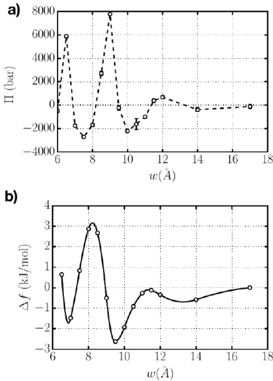
Figure 12. (a) The hydration pressure \Pi as a function of the slit-pore width w at T = 300 K is vanishing at perfect and intermediate size values of w (see text), is maximum at undersized values of w and minimum (negative) at oversized values of w . (b) Work, per confined water molecule, performed to approach the graphene plates from w_0 to w , as a function of the separation w , for T = 300 K. Adapted from Ref. 196 with permission from Elsevier.
