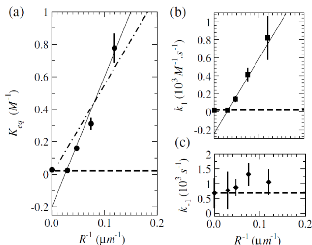
Figure 4. Results from fluorescence imaging for the reactivity parameters of a bimolecular transformation inside micro-meter-size water droplets. The panels show the effect of compartment dimensions on the equilibrium constant K_{eq} (a), on the forward reaction rate k_1 (b), and on the backward reaction rate k_{-1} (c). K_{eq} and k_1 exhibit a linear dependence with the inverse radius of the droplet, which can be explained on the basis of a reaction-adsorption mechanism. Reproduced from Ref. 105 with permission of the American Physical Society.
