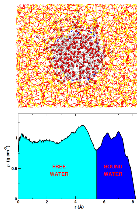
Figure 7. Upper Panel: snapshot of the MCM-41 system projected in two dimension at T = 300 K. The box length is L = 4.278 nm and the diameter of the cylindrical pore is 1.5 nm. The acidic hydrogens are the inner, darker sticks, the water molecules are the dark and light spheres, and the silica molecules are the outer sticks. Figure from Ref. [202]. Bottom Panel: density profile of oxygen atoms of water confined in MCM-41 along the pore radius with origin at the center of the pore at T = 300 K. The density of the free water is around 1.0 \text{ g/cm}^3 . Reprinted with permission from Ref. 173. Copyright 2017 American Chemical Society.
