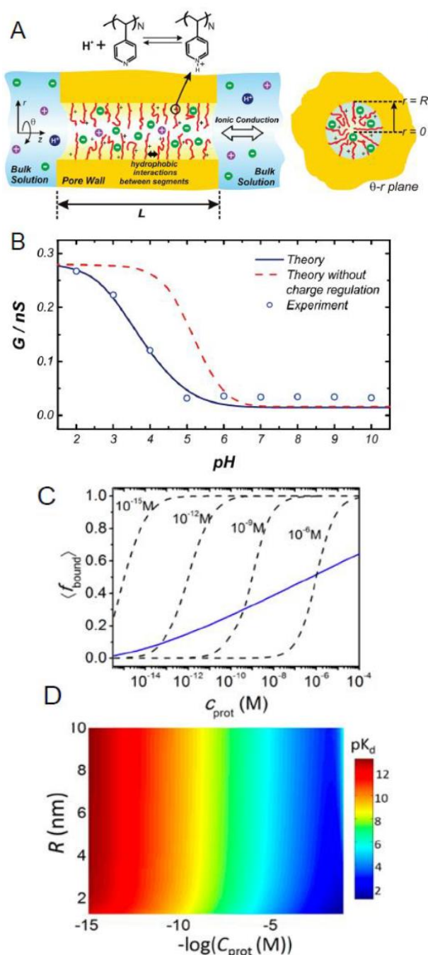
Figure 23. Shifted equilibria of chemical reactions in polymer-coated nanopores. (A) Schematic representation of the polyelectrolyte brush modified long nanopore. The inner surface of the pore is modified with end-tethered chains of poly(4-vinyl pyridine). (B) Comparison between experiment and molecular theory on the pH-dependent conductivity. Reprinted with permission from Ref. 497. (C) Molecular theory prediction of average fraction of bound ligands inside a nanopore as a function of the molar concentration of the proteins in bulk solution (solid blue line), in comparison with the predictions of the Langmuir isotherm for different values of the dissociation constant (black dashed lines). (D) Apparent dissociation constant as a function of the pore radius and the molar concentration of the proteins in bulk solution. Reprinted with permission from Ref. 525. Copyright 2015 American Chemical Society.
