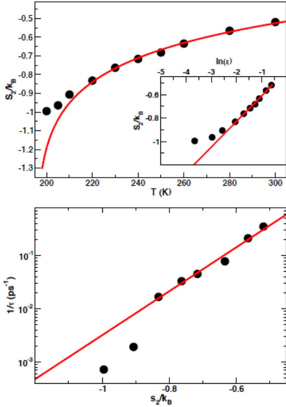
Figure 9. Upper panel: two body entropy, s_2 for the free water confined in MCM-41 silica as a function of the temperature. The continuous red line is fit to the MCT behavior in Eqn. 13 with T_C = 195 K. In the inset the data are shown as function of \ln \epsilon , where \epsilon = (T - T_C)/T_C . Bottom panel: inverse of the \alpha -relaxation time, \tau , as function of the two-body entropy, s_2 for the free water confined in MCM-41 silica. The red curve is the fit to Eqn. 10. Adapted from Ref. 172, with the permission of AIP Publishing.
