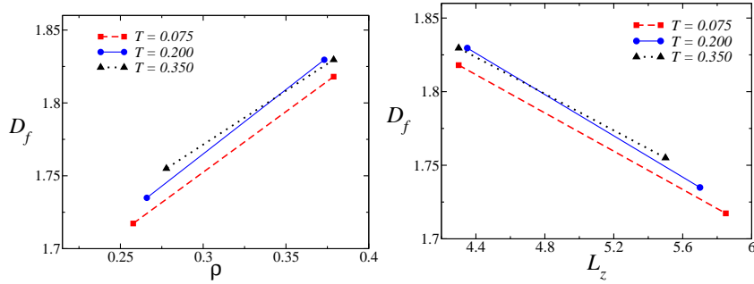
Figure 3: (a) Fractal dimension as function of (a) total density and (b) separation of plates for transition at high densities.
