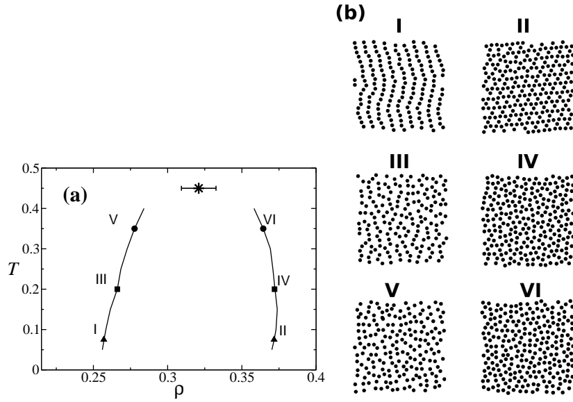
Figure 2: (a) Temperature versus total density phase diagram for high densities. The star represents the critical point at T_c = 0.450 and \rho_c = 0.321 . The solid lines delineate the coexistence region between liquid-crystal and hexagonal solid phases. The triangles, squares and circles are isochores at T = 0.075 , 0.200 and 0.350 , respectively, and densities \rho_{I,III,V} \approx 0.260 , \rho_{II,IV,VI} \approx 0.370 . The corresponding snapshots of the contact layer are shown in (b). More details in the text.
